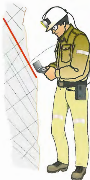
Measurement of Joint Orientation Using Field Compass
