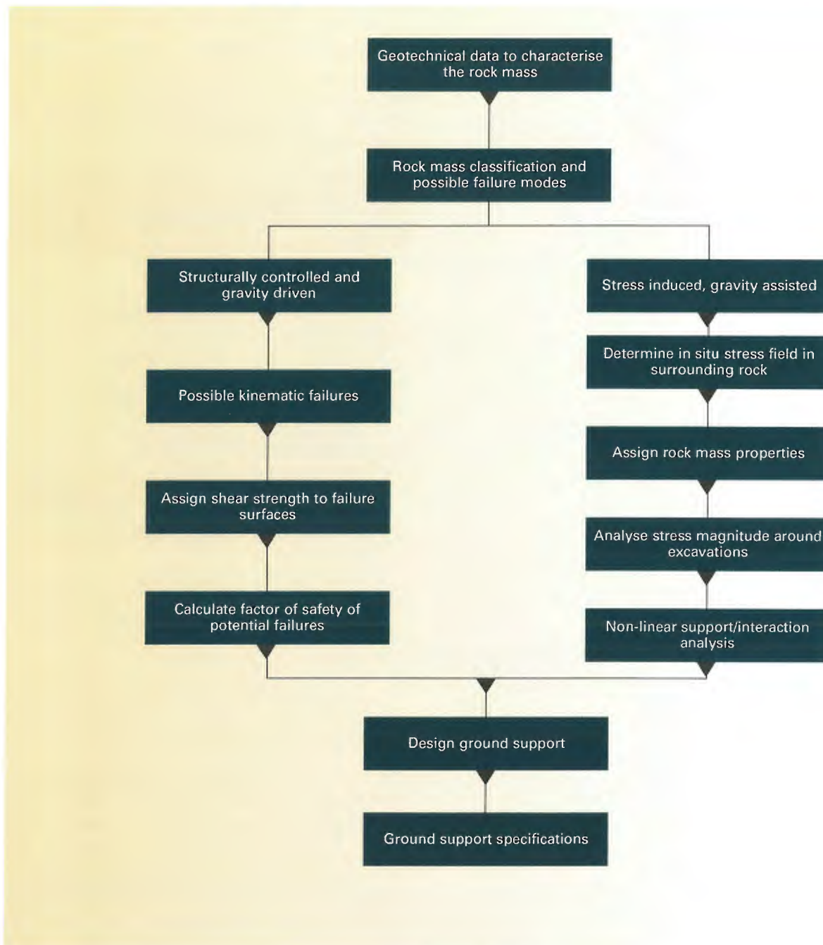
Figure 49: Flowchart describing a process for designing ground support (Modified after Hoek, Kaiser and Bawden 1995)
