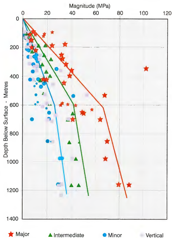
Figure 11: Compilation of stress measurement data from the Kalgoorlie-Kambalda region showing the magnitude of the principal stresses as a function of depth (Reproduced after Lee et al 1999)
