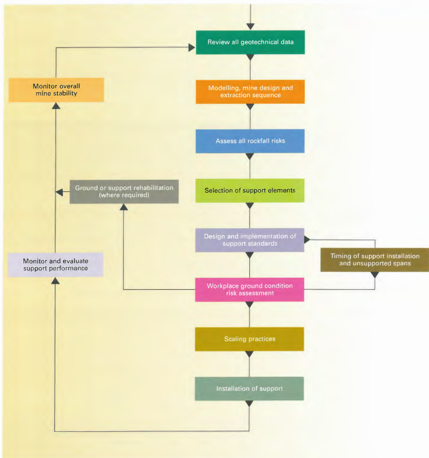
Figure 48: Process for the development and implementation strategy of ground support standards
