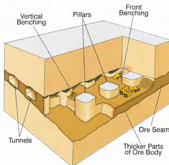
Figure 36: Illustration of a generic room and pillar operation showing mine production activities within the stope (Reproduced after Hamrin 2001)
