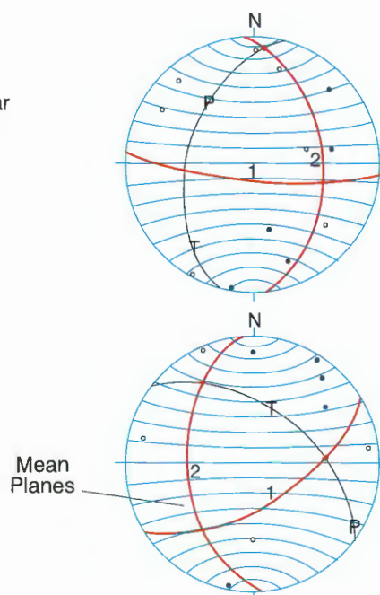
Figure 4: Illustration of the process commonly used to collect, record and present structural data (Reproduced after Hutchinson and Diederichs 1996)
